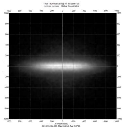
lighting spot
